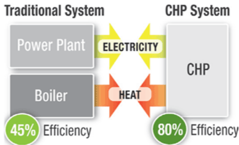
CHP Process Flow Diagram
